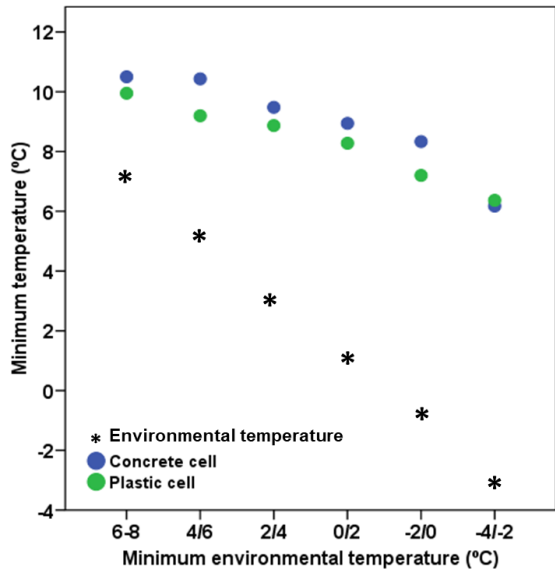
Fig: Ambient and internal cell minimum temperature in cold season
